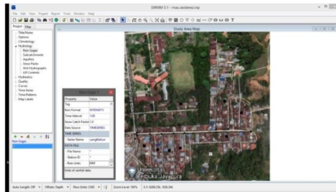
Fig 11: Display rain gauge
