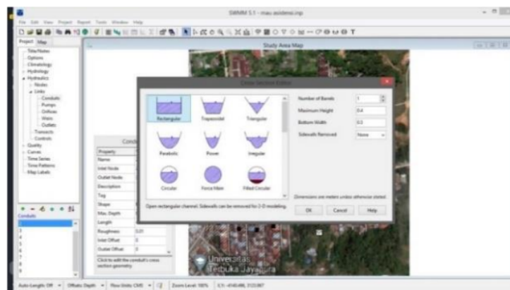
Fig 7: Channel shape selection (conduit)
