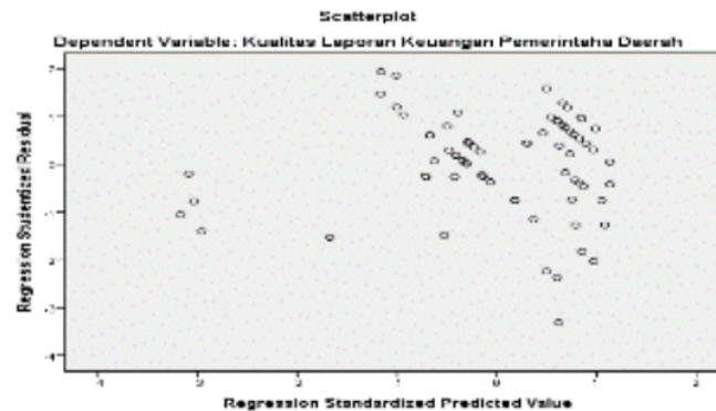
Figure 2. Heteroscedasticity Testing Results
