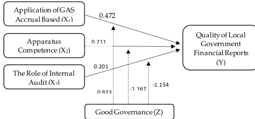
Figure 3. Research Model with MRA Coefficient
