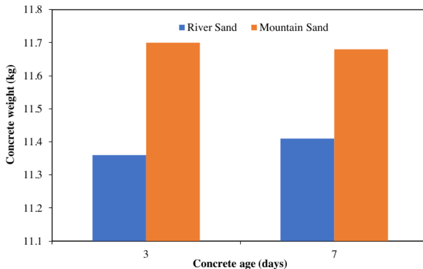
Fig 3: Weight of concrete
