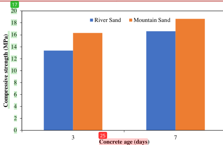
Fig 4: Compressive strength of concrete
