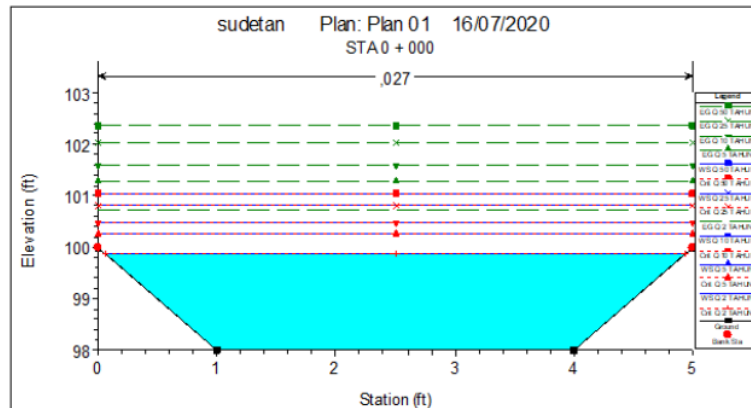
Figure 1. Sudetan HEC RAS analysis
